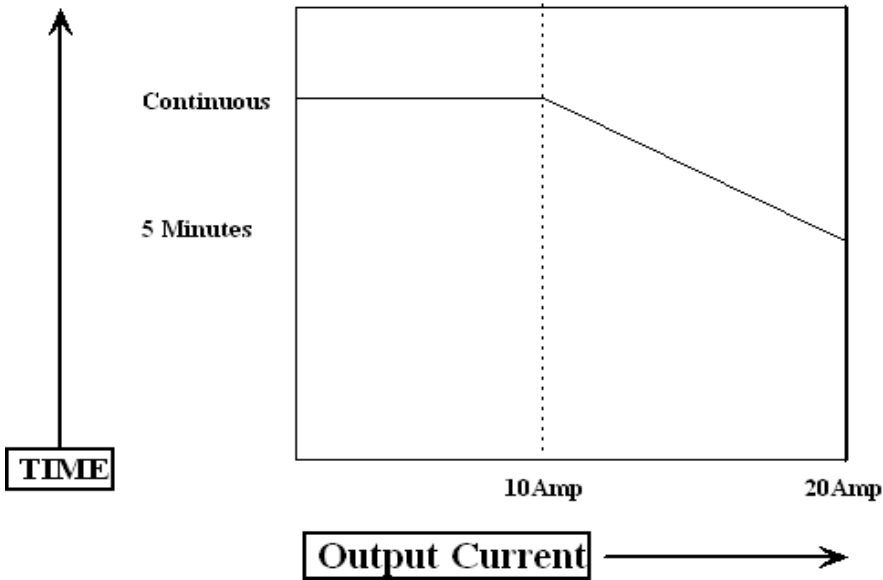
Graph 5* : Operating time on 20A range with current into a short circuit at 20°C Continuous current available up to 10A output.
